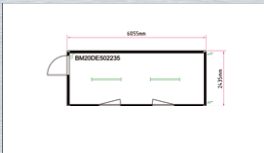
Grundriss 20' BM Standard
